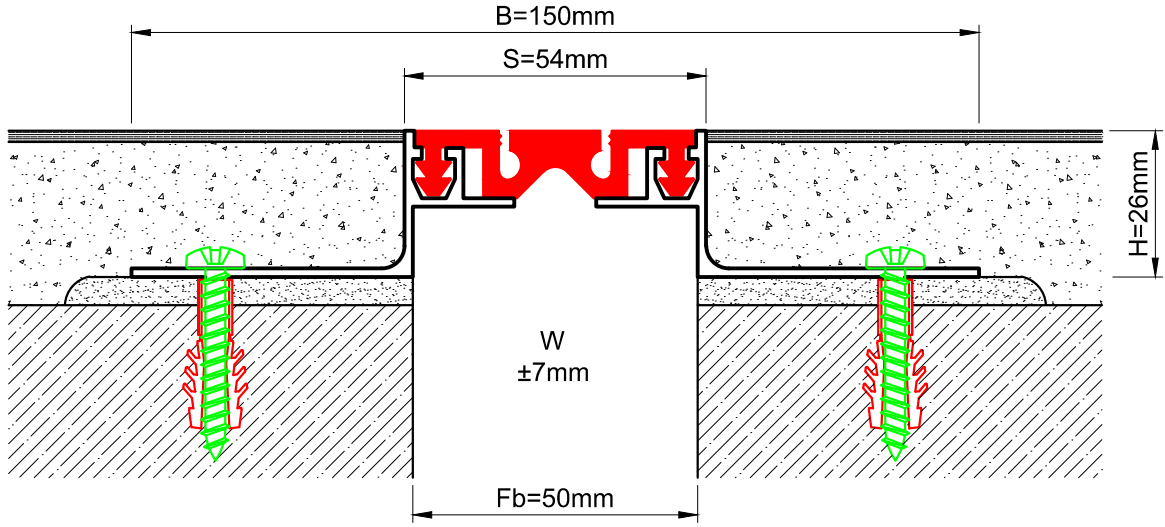
AS A246L-050 H=26mm
