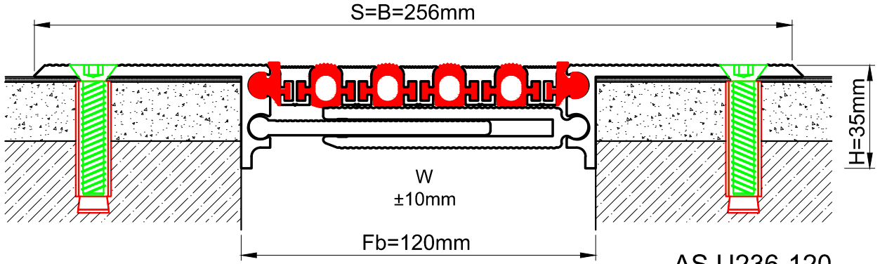
AS U236-120 H=35mm
