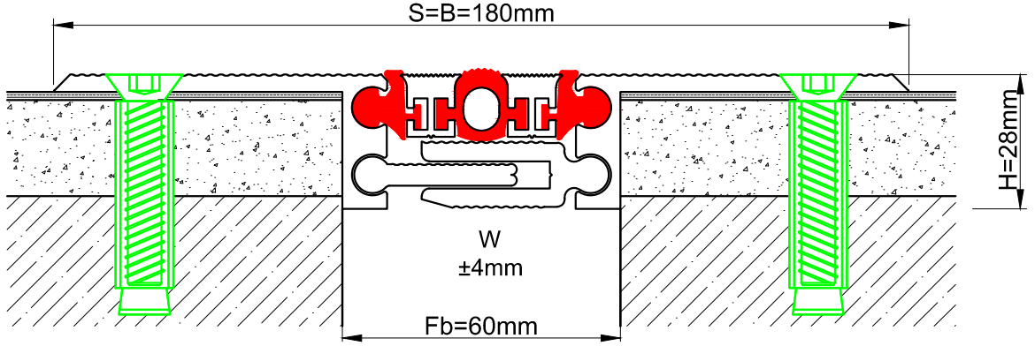
AS U236-060 H=28mm
