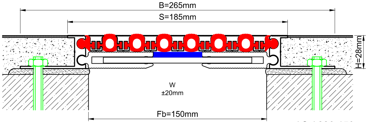
AS A226-150 H=28mm
