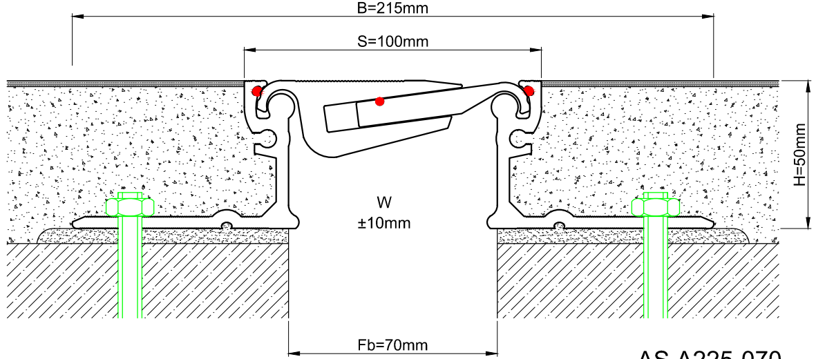
AS A225-070 H=50mm
